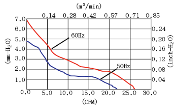
SK838 P-Q Curves
