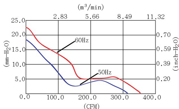
SK160 P-Q Curves
