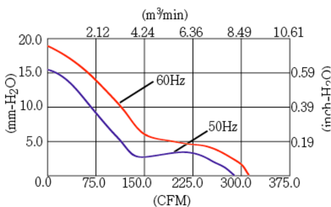
SK170 P-Q Curves
